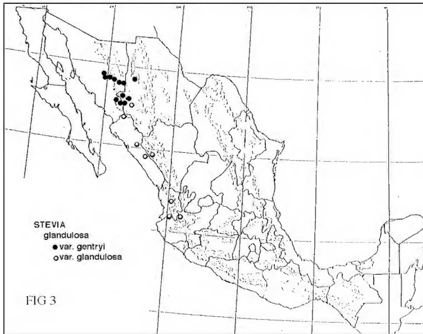
Fig. 3. Distribution of Stevia glandulosa .
